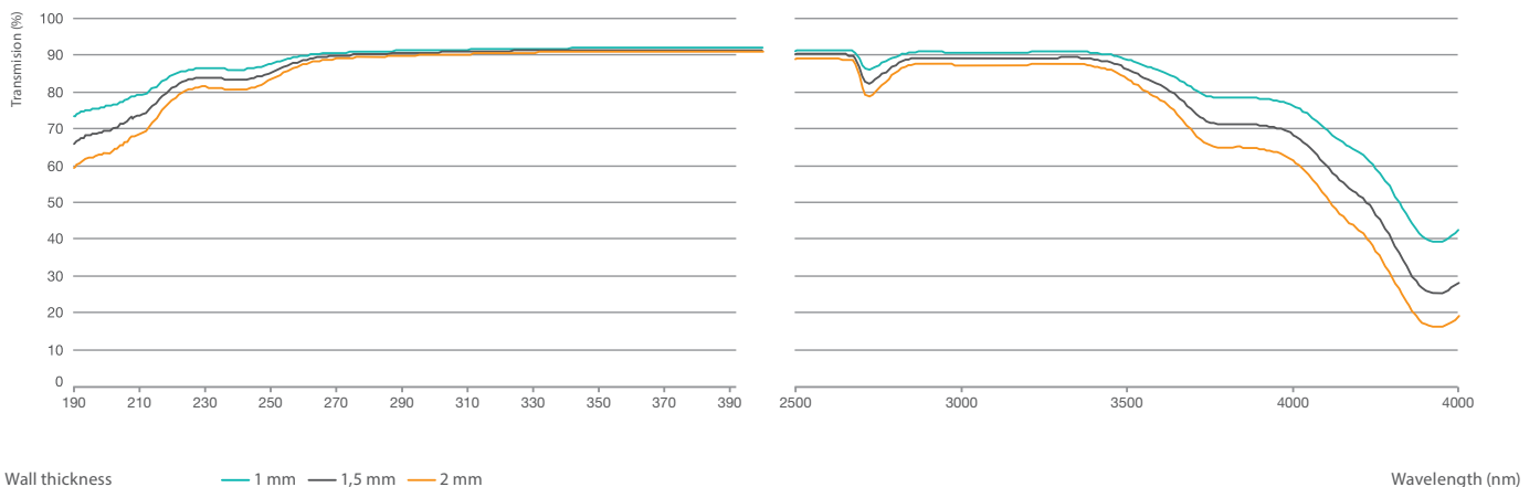
Transmission curve
