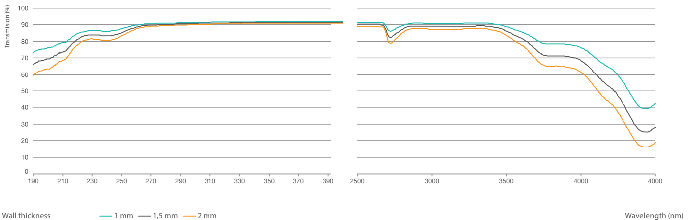
Transmission curve
