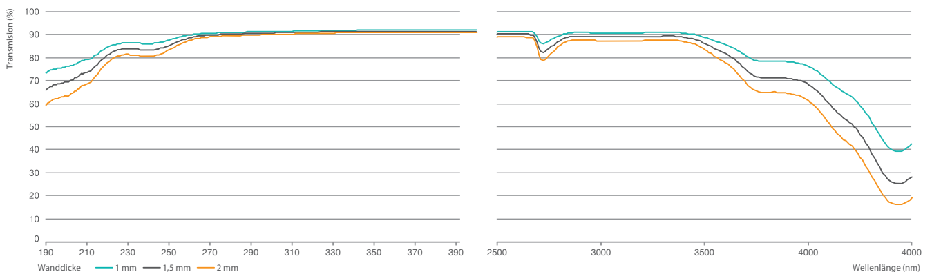
Transmissionskurve
